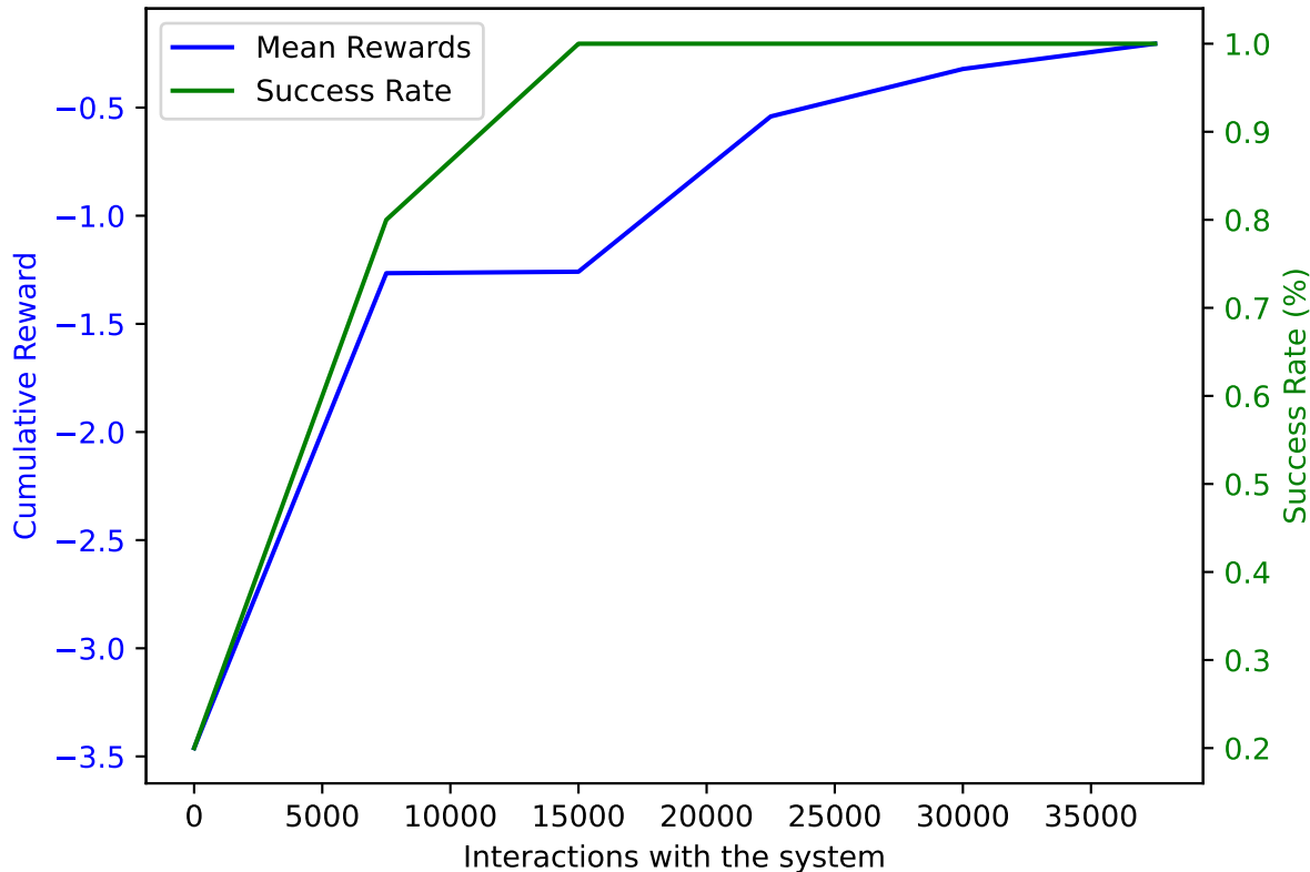
PPO on AWAKE with DoF: 1 and trained on 37500 samples averaged over 10 validation episodes
