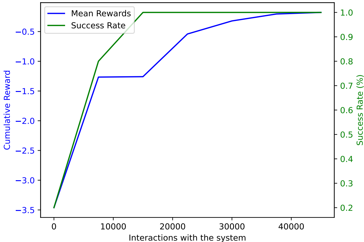
PPO on AWAKE with DoF: 1 and trained on 45000 samples averaged over 10 validation episodes
