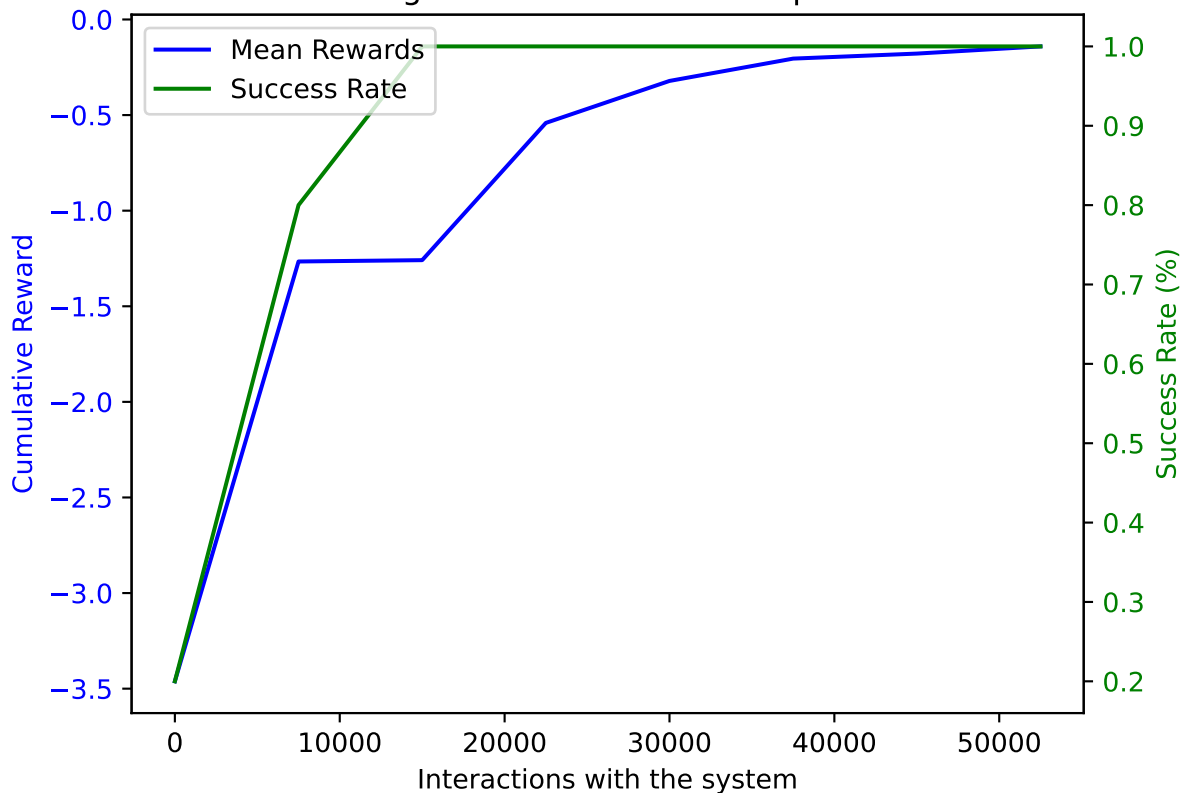
PPO on AWAKE with DoF: 1 and trained on 52500 samples averaged over 10 validation episodes
