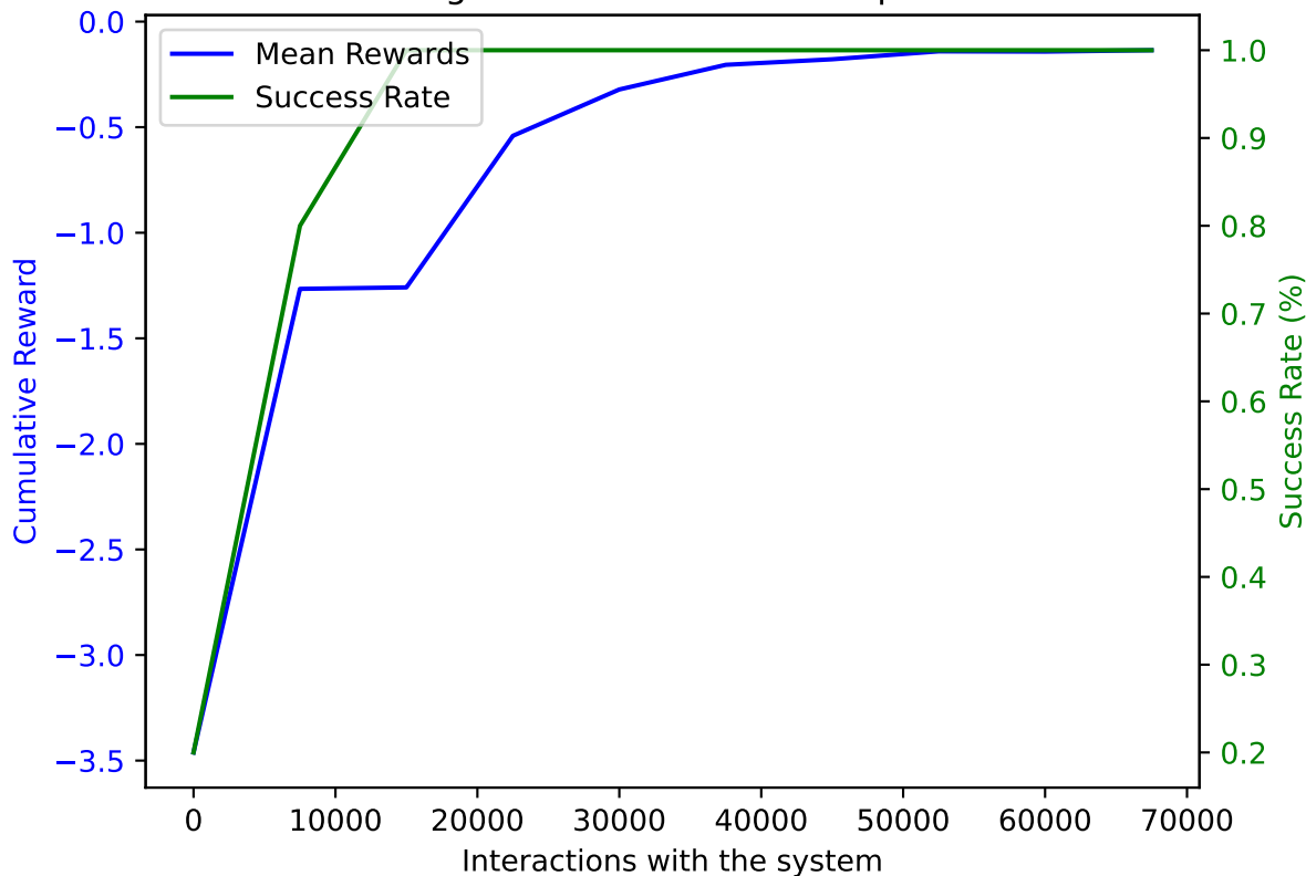
PPO on AWAKE with DoF: 1 and trained on 67500 samples averaged over 10 validation episodes
