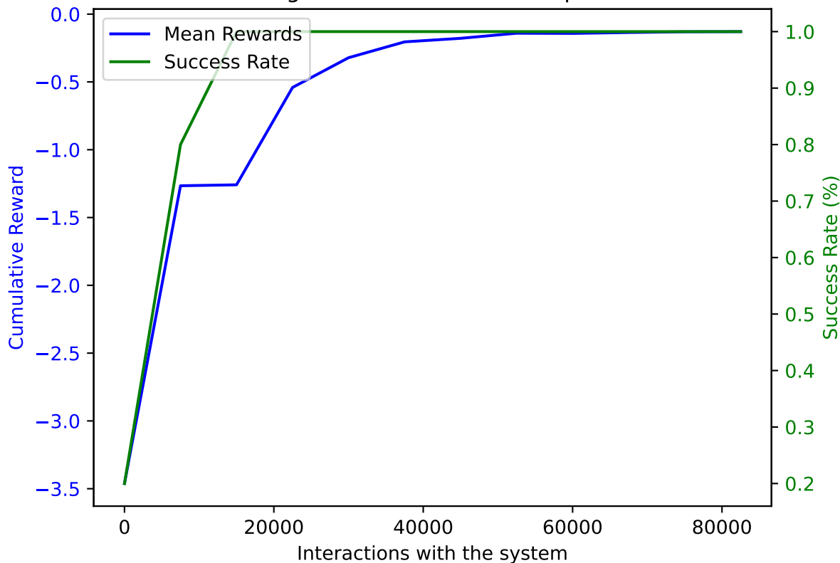
PPO on AWAKE with DoF: 1 and trained on 82500 samples averaged over 10 validation episodes
