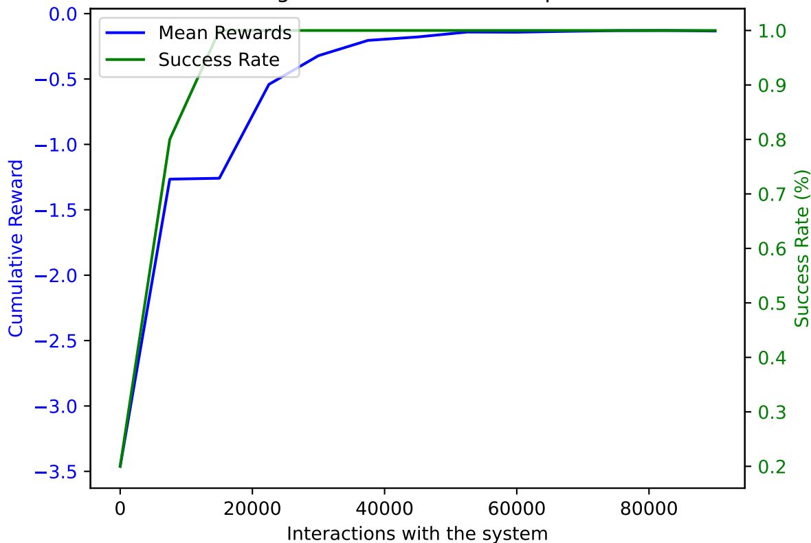
PPO on AWAKE with DoF: 1 and trained on 90000 samples averaged over 10 validation episodes
