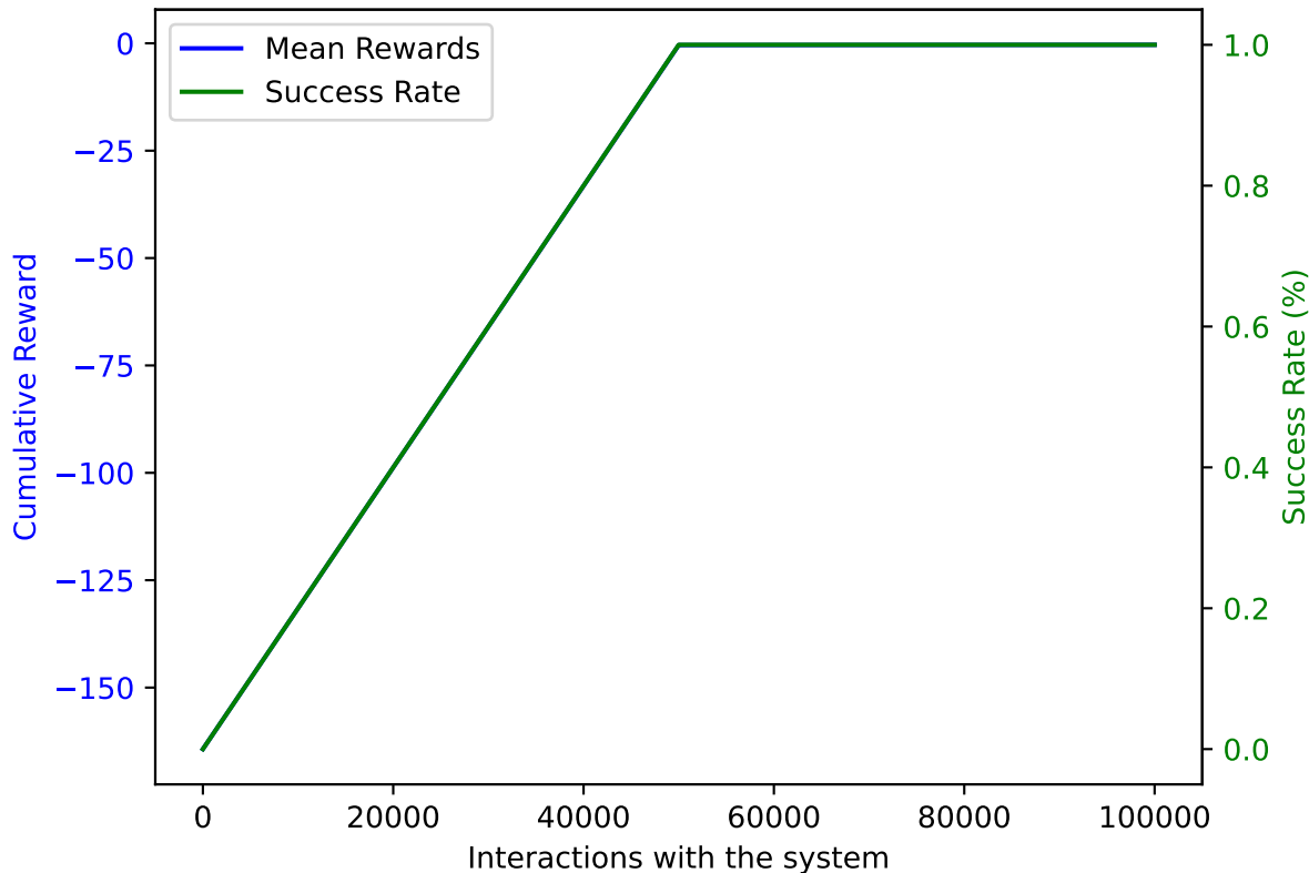
PPO on AWAKE with DoF: 2 and trained on 100000 samples averaged over 10 validation episodes
