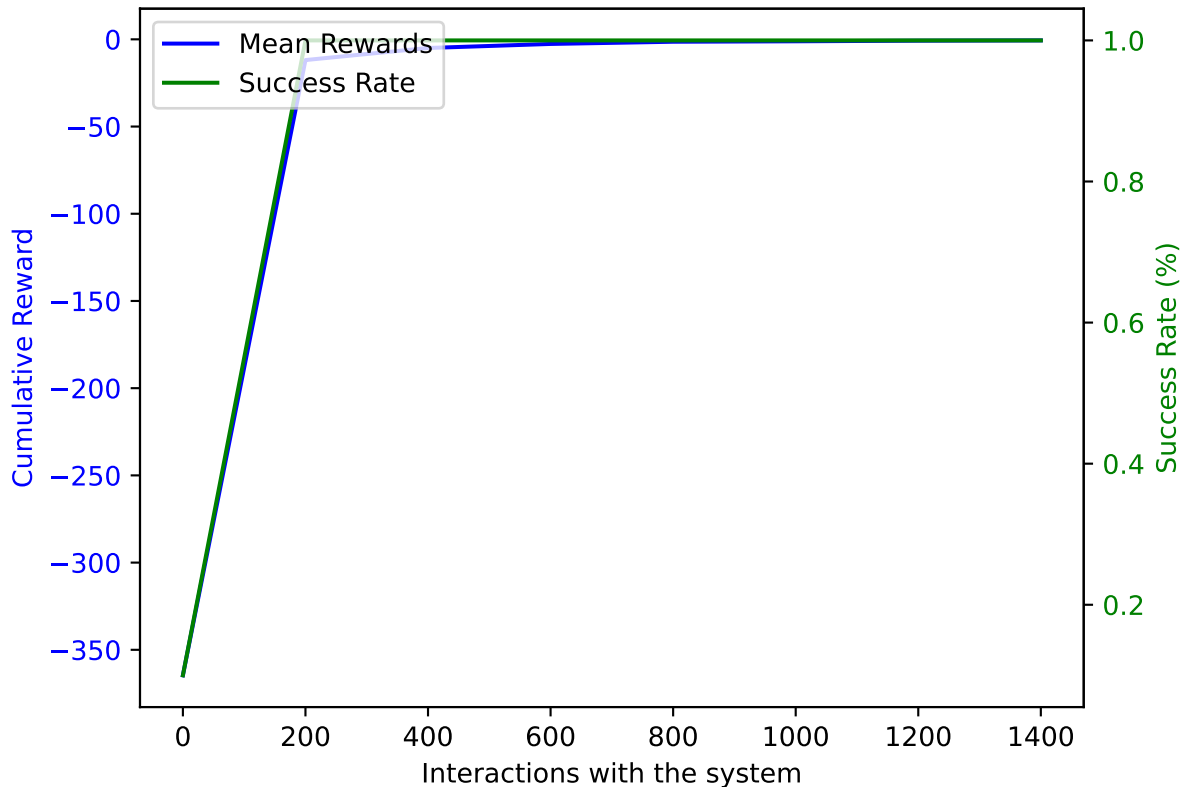
PPO on AWAKE with DoF: 2 and trained on 1400 samples averaged over 10 validation episodes
