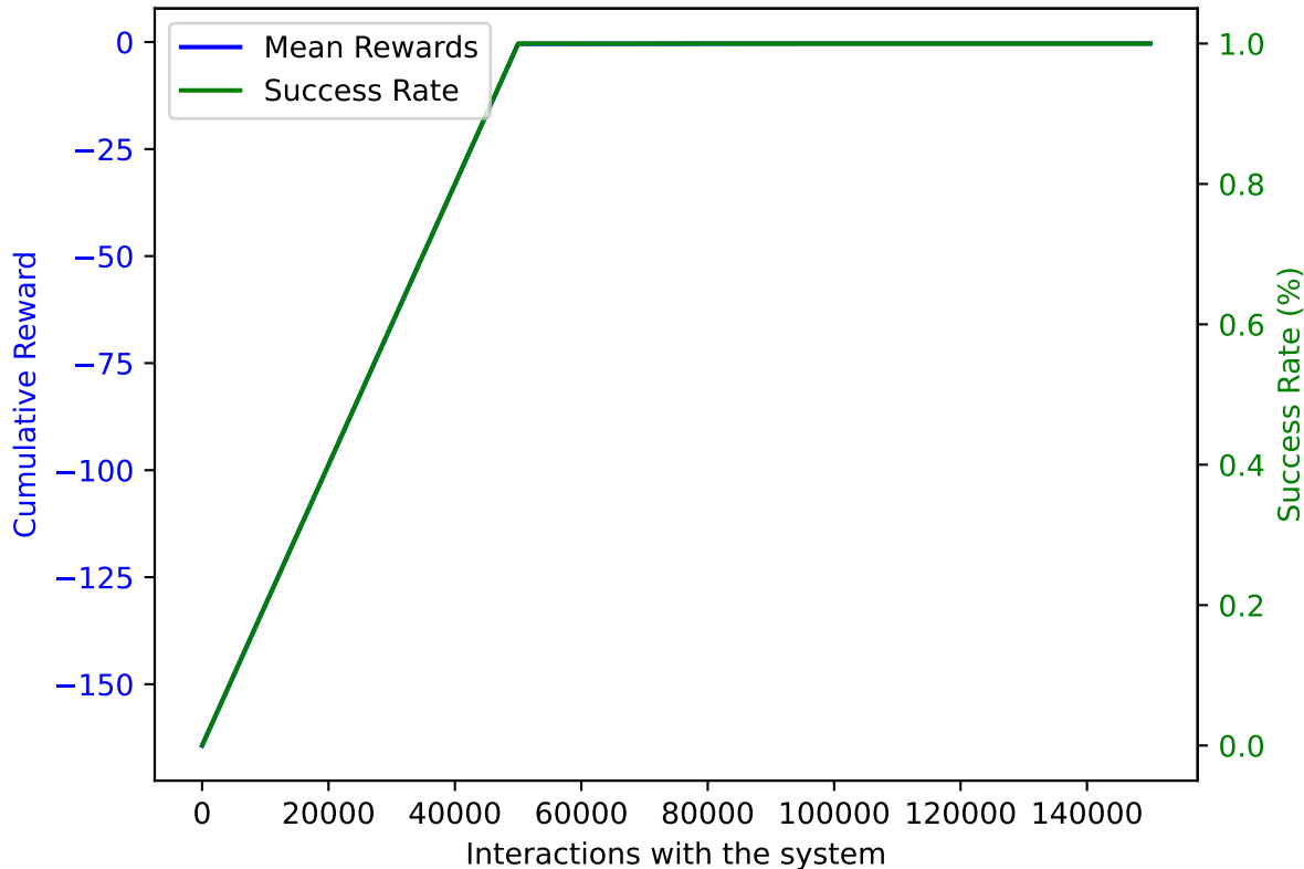
PPO on AWAKE with DoF: 2 and trained on 150000 samples averaged over 10 validation episodes
