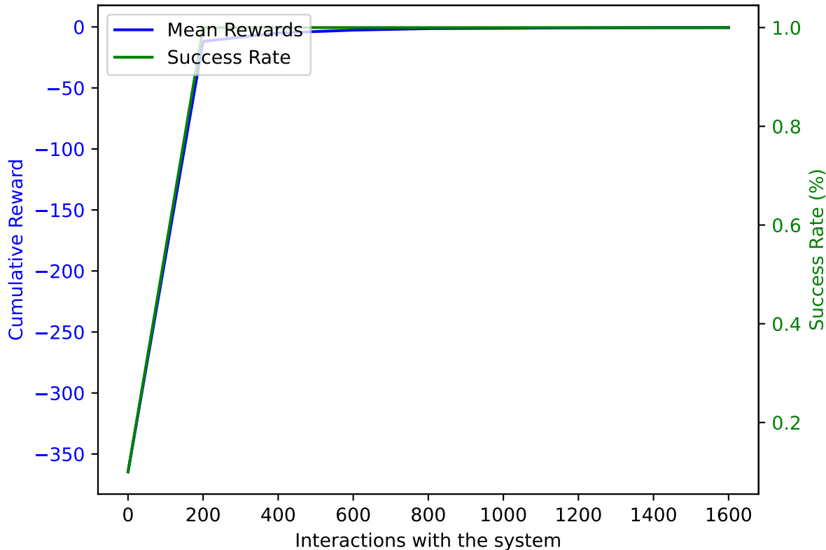
PPO on AWAKE with DoF: 2 and trained on 1600 samples averaged over 10 validation episodes
