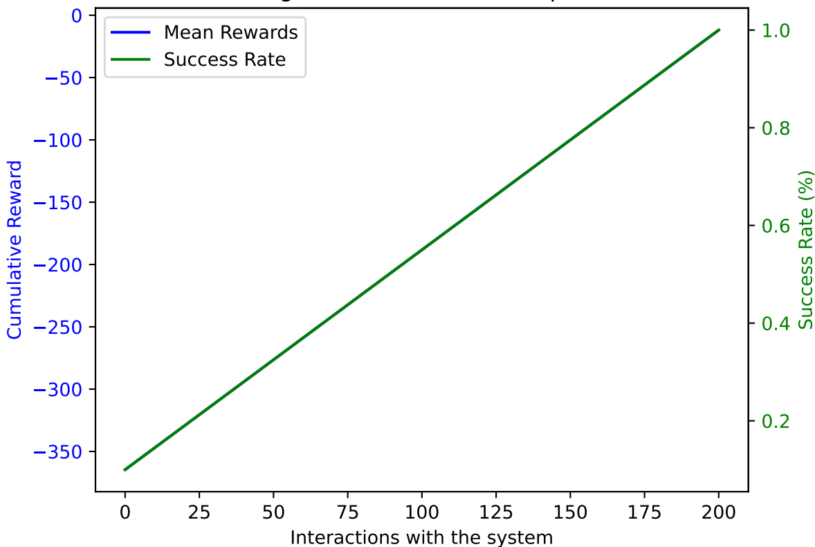
PPO on AWAKE with DoF: 2 and trained on 200 samples averaged over 10 validation episodes
