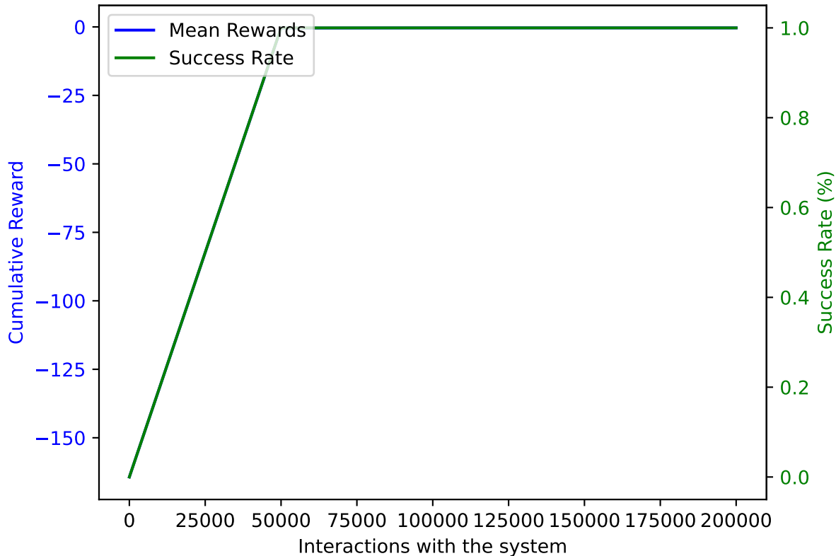
PPO on AWAKE with DoF: 2 and trained on 200000 samples averaged over 10 validation episodes
