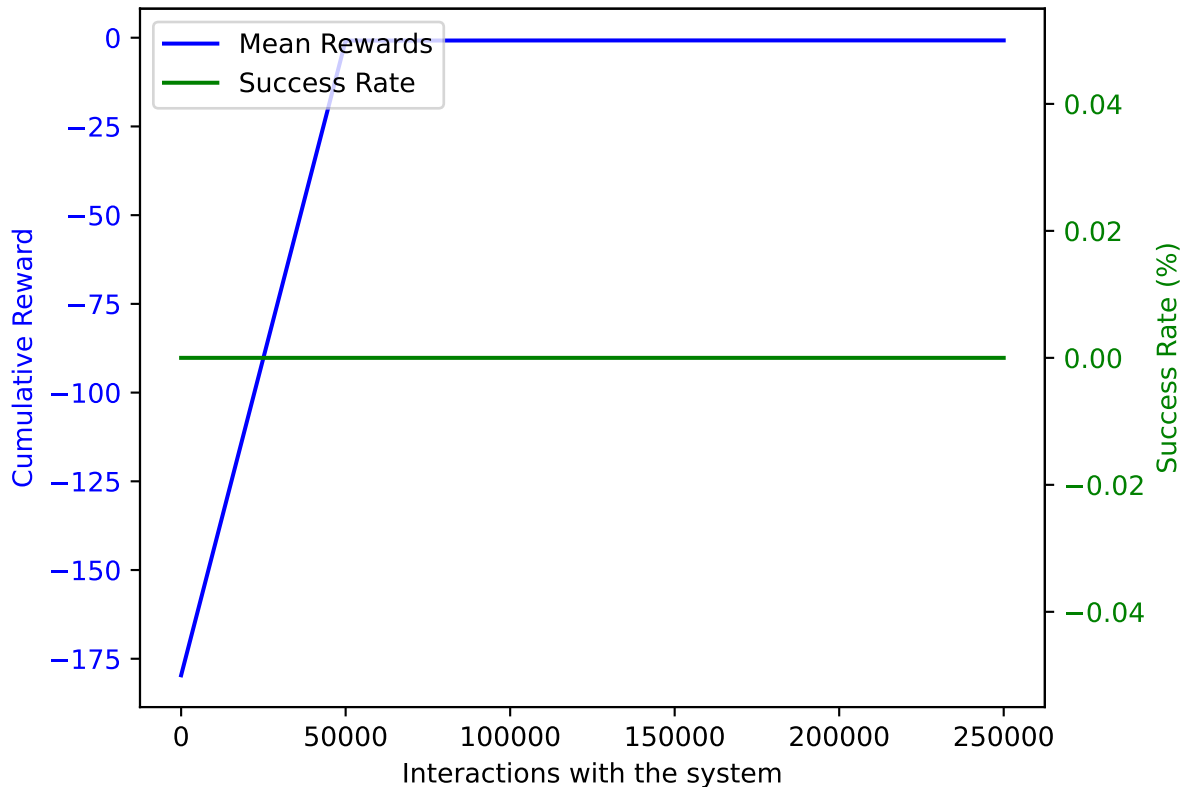
PPO on AWAKE with DoF: 2 and trained on 250000 samples averaged over 10 validation episodes
