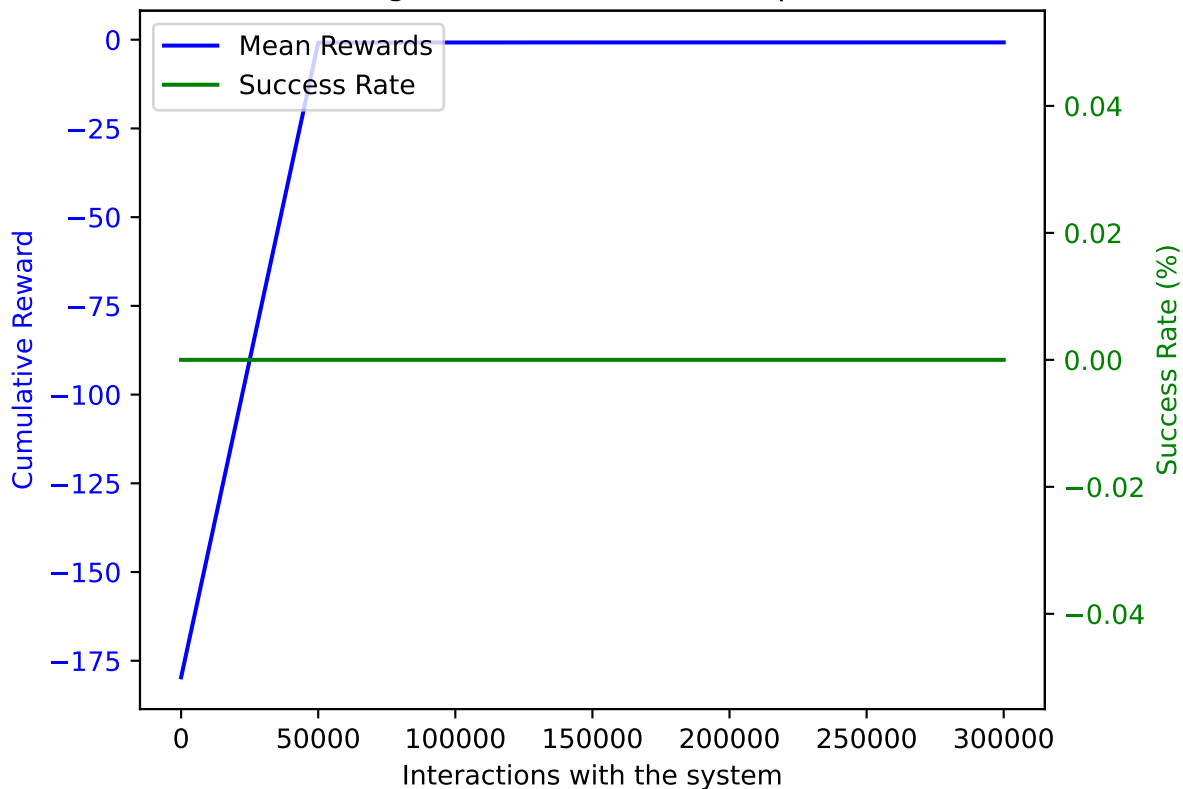
PPO on AWAKE with DoF: 2 and trained on 300000 samples averaged over 10 validation episodes
