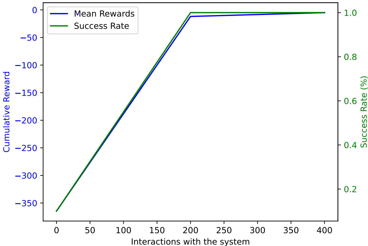
PPO on AWAKE with DoF: 2 and trained on 400 samples averaged over 10 validation episodes
