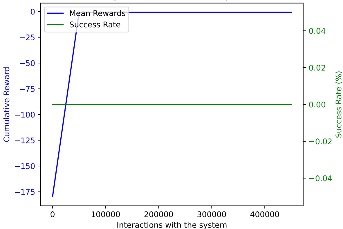
PPO on AWAKE with DoF: 2 and trained on 450000 samples averaged over 10 validation episodes
