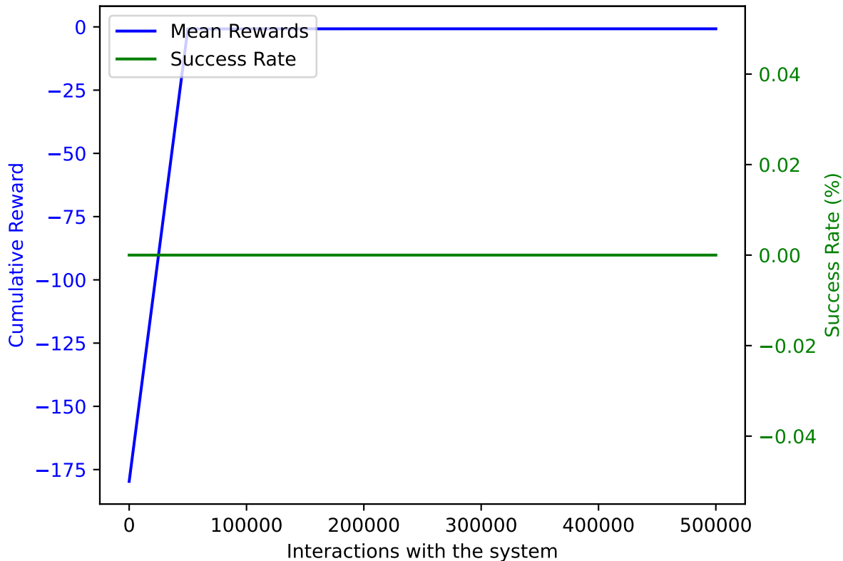
PPO on AWAKE with DoF: 2 and trained on 500000 samples averaged over 10 validation episodes
