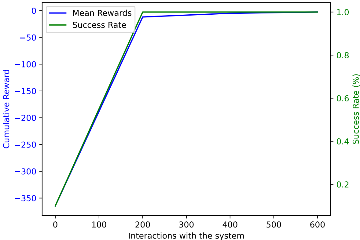
PPO on AWAKE with DoF: 2 and trained on 600 samples averaged over 10 validation episodes
