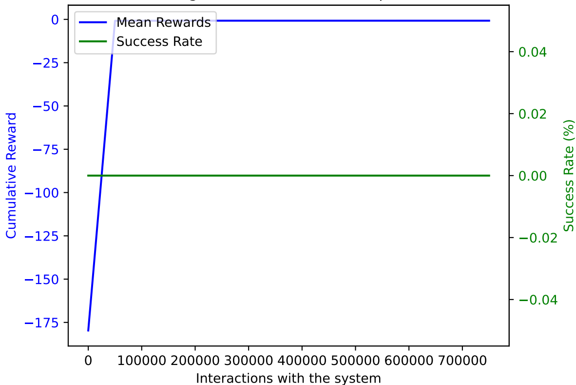
PPO on AWAKE with DoF: 2 and trained on 750000 samples averaged over 10 validation episodes
