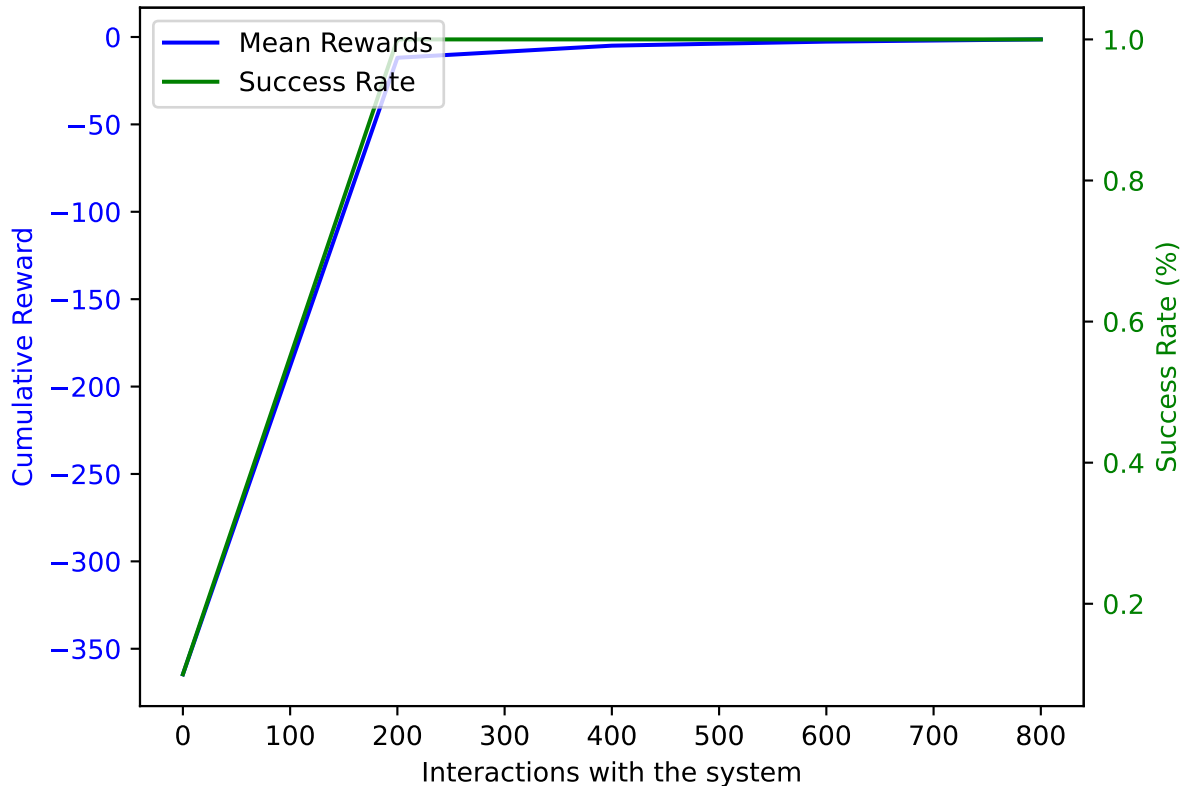
PPO on AWAKE with DoF: 2 and trained on 800 samples averaged over 10 validation episodes
