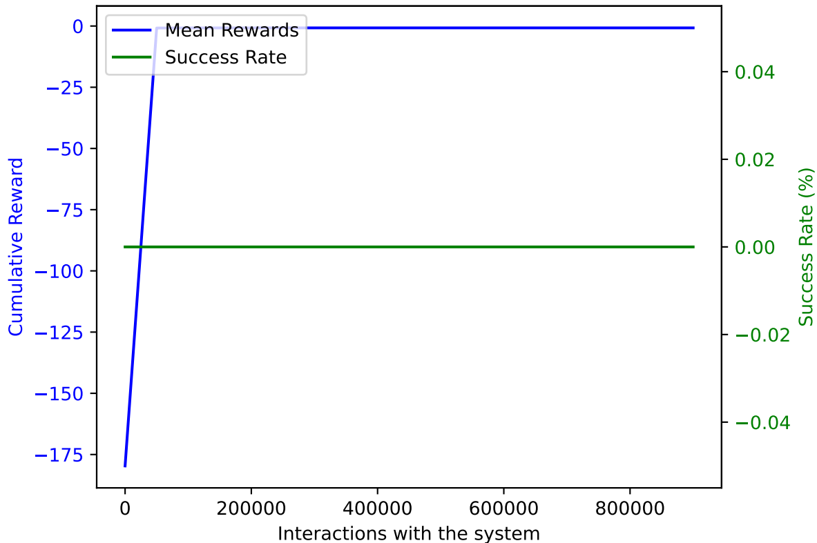
PPO on AWAKE with DoF: 2 and trained on 900000 samples averaged over 10 validation episodes
