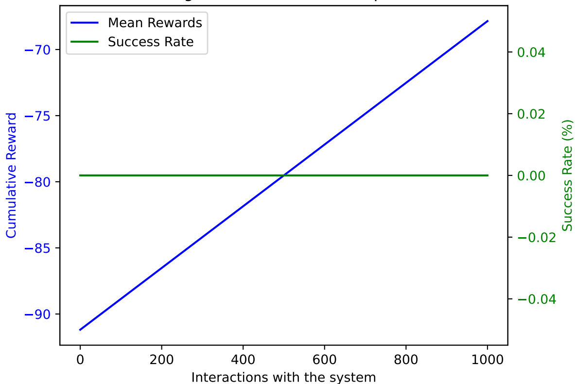
PPO on AWAKE with DoF: 5 and trained on 1000 samples averaged over 10 validation episodes
