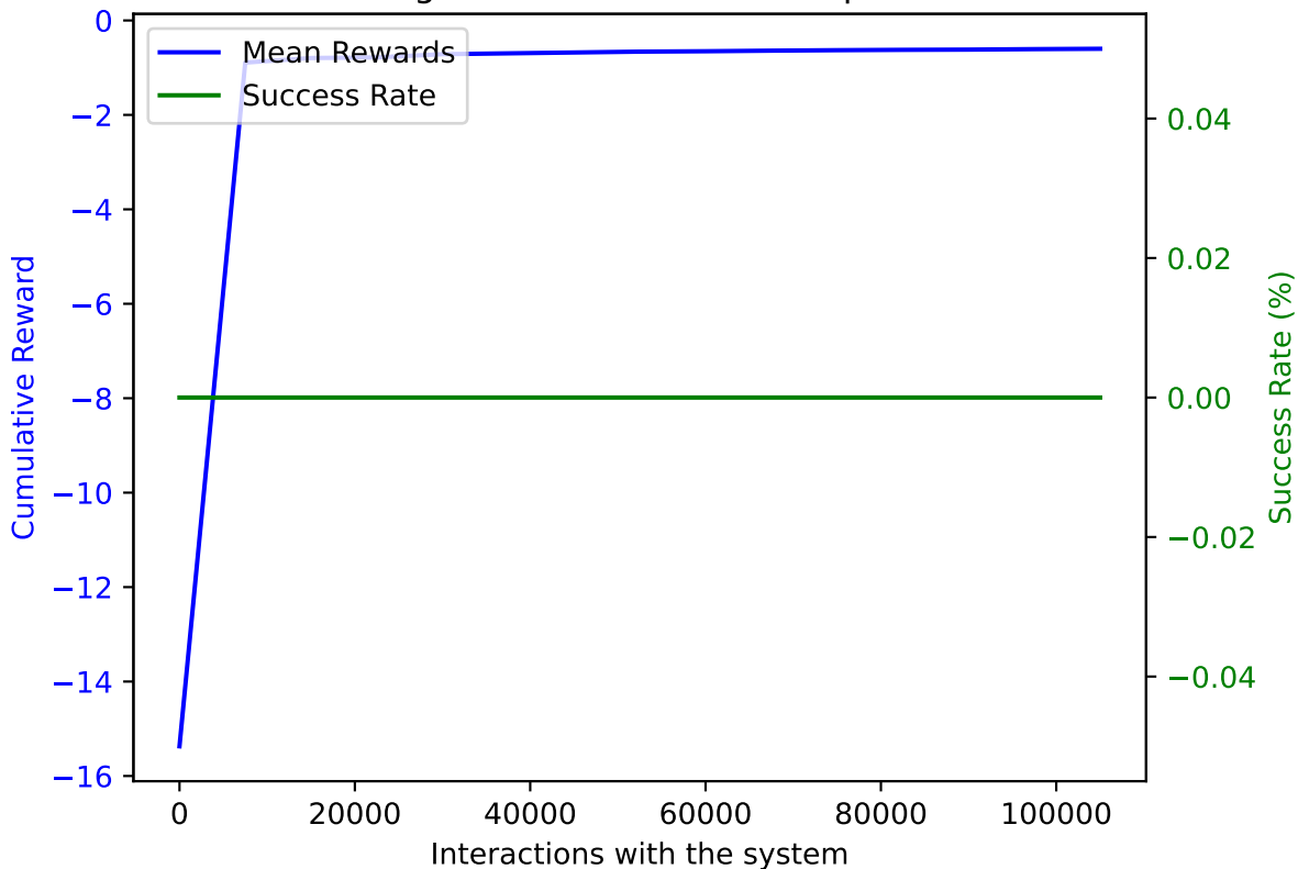
PPO on AWAKE with DoF: 5 and trained on 105000 samples averaged over 10 validation episodes
