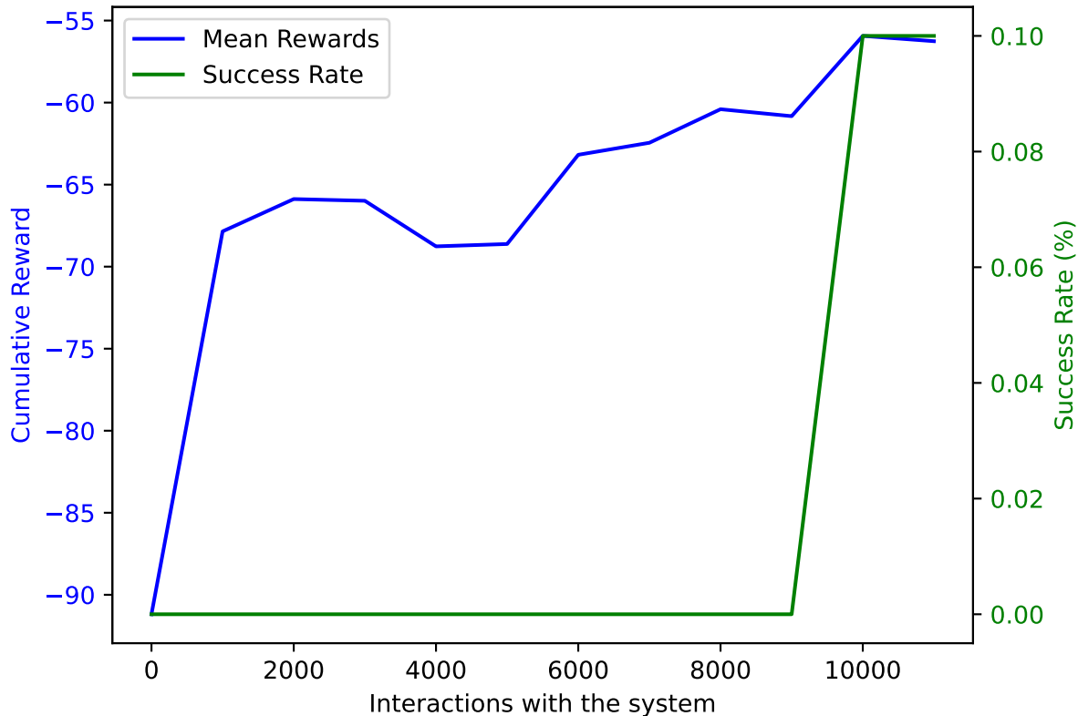
PPO on AWAKE with DoF: 5 and trained on 11000 samples averaged over 10 validation episodes
