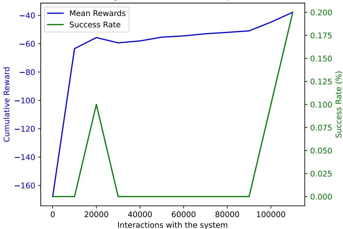
PPO on AWAKE with DoF: 5 and trained on 110000 samples averaged over 10 validation episodes
