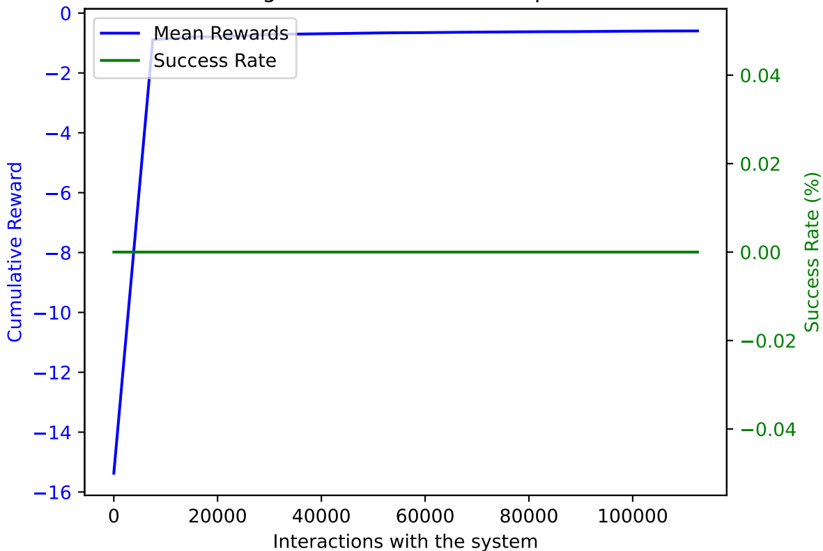
PPO on AWAKE with DoF: 5 and trained on 112500 samples averaged over 10 validation episodes
