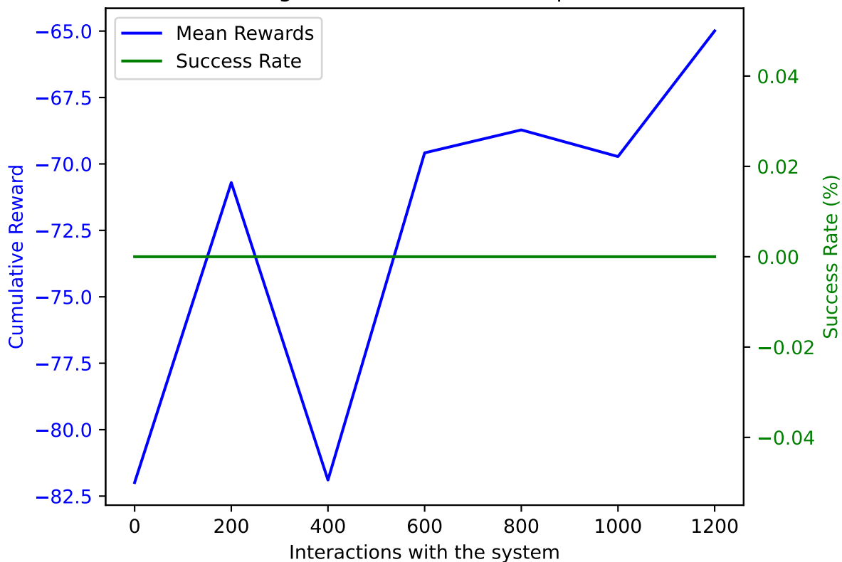
PPO on AWAKE with DoF: 5 and trained on 1200 samples averaged over 10 validation episodes
