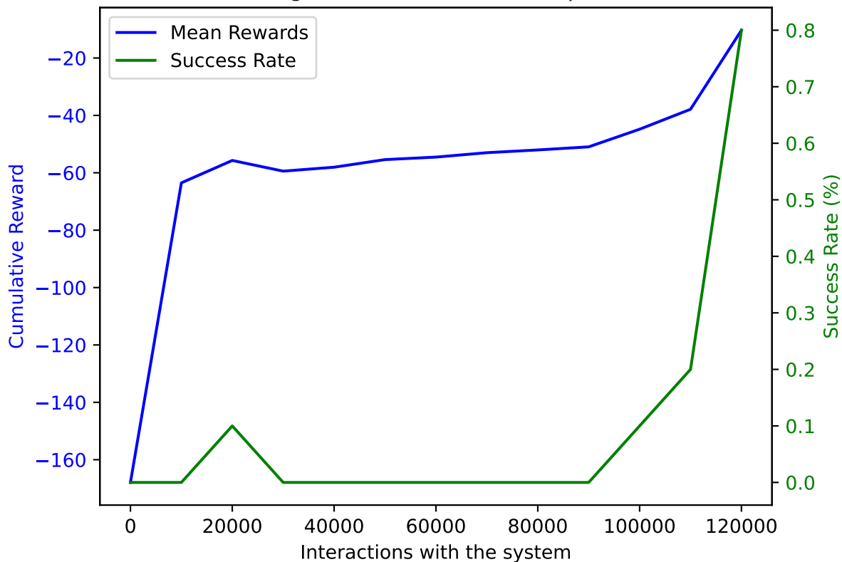
PPO on AWAKE with DoF: 5 and trained on 120000 samples averaged over 10 validation episodes
