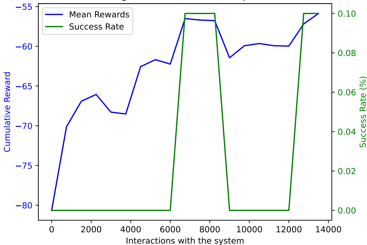
PPO on AWAKE with DoF: 5 and trained on 13500 samples averaged over 10 validation episodes
