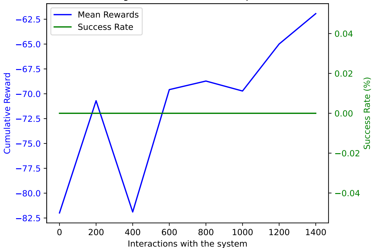
PPO on AWAKE with DoF: 5 and trained on 1400 samples averaged over 10 validation episodes
