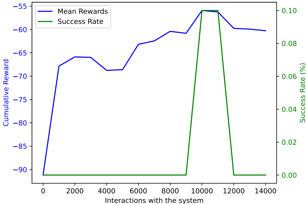
PPO on AWAKE with DoF: 5 and trained on 14000 samples averaged over 10 validation episodes
