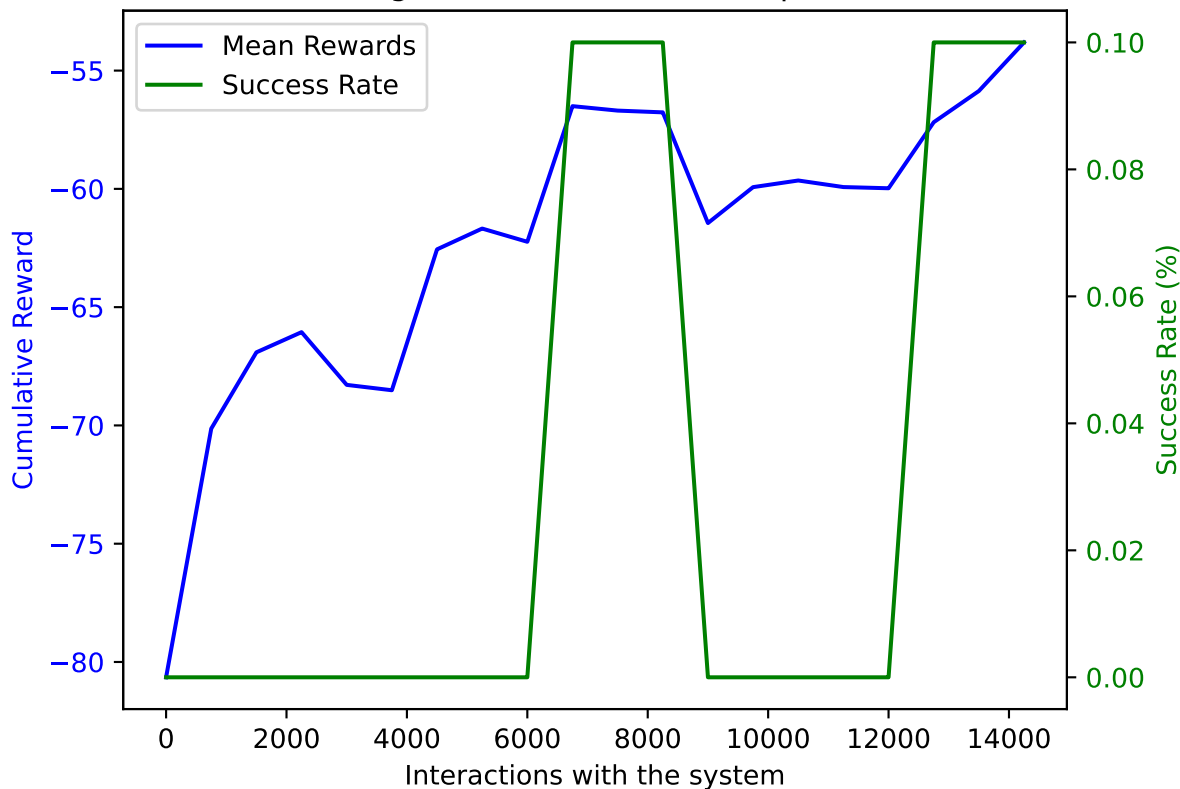
PPO on AWAKE with DoF: 5 and trained on 14250 samples averaged over 10 validation episodes
