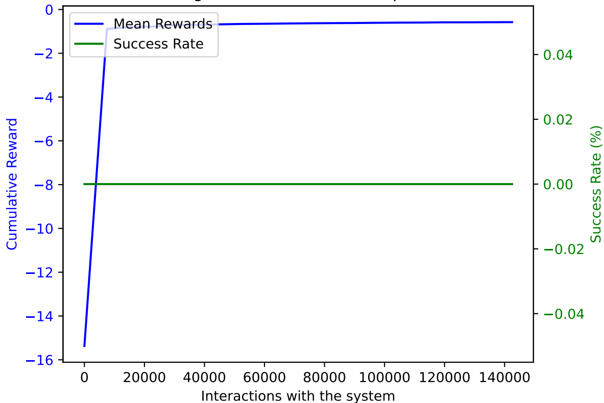
PPO on AWAKE with DoF: 5 and trained on 142500 samples averaged over 10 validation episodes
