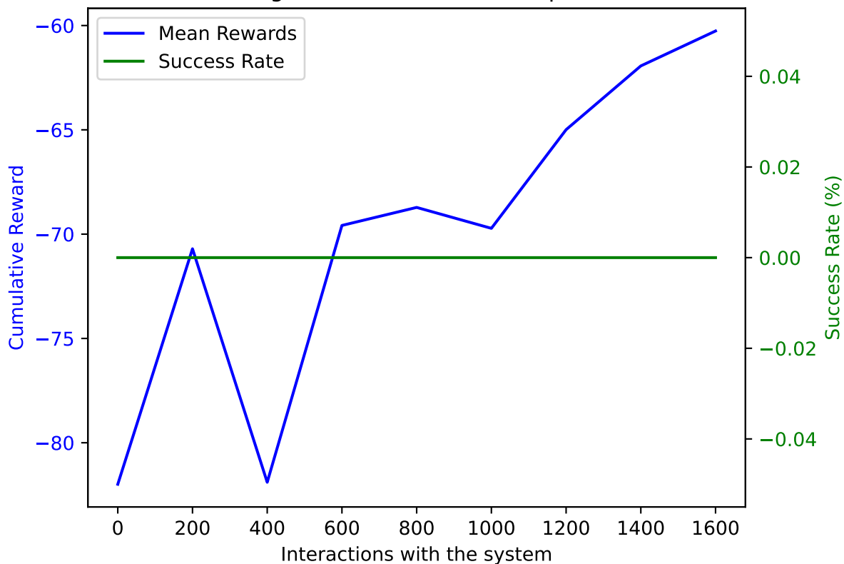
PPO on AWAKE with DoF: 5 and trained on 1600 samples averaged over 10 validation episodes
