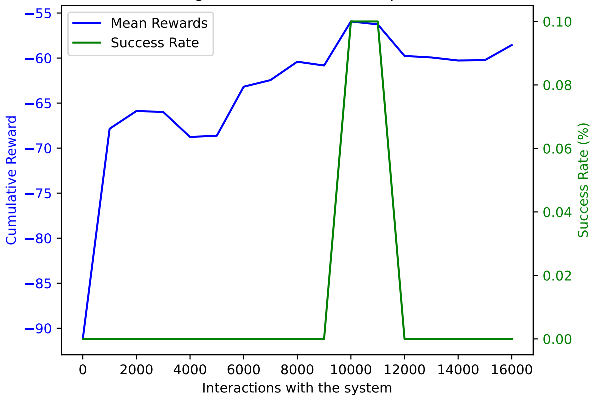
PPO on AWAKE with DoF: 5 and trained on 16000 samples averaged over 10 validation episodes
