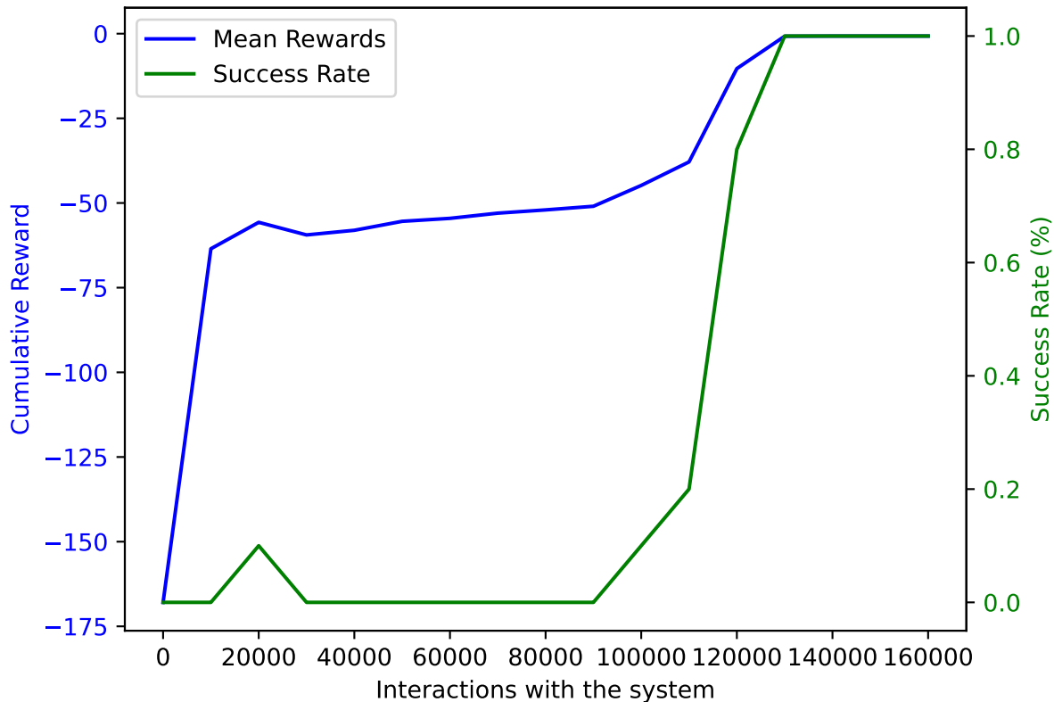
PPO on AWAKE with DoF: 5 and trained on 160000 samples averaged over 10 validation episodes
