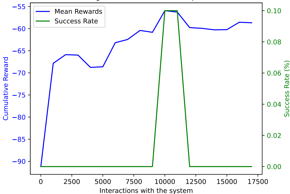
PPO on AWAKE with DoF: 5 and trained on 17000 samples averaged over 10 validation episodes
