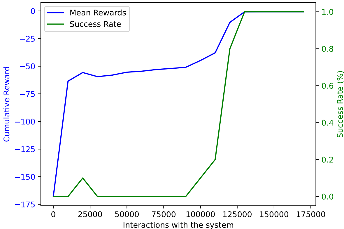
PPO on AWAKE with DoF: 5 and trained on 170000 samples averaged over 10 validation episodes
