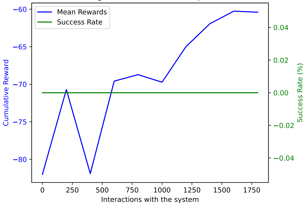
PPO on AWAKE with DoF: 5 and trained on 1800 samples averaged over 10 validation episodes
