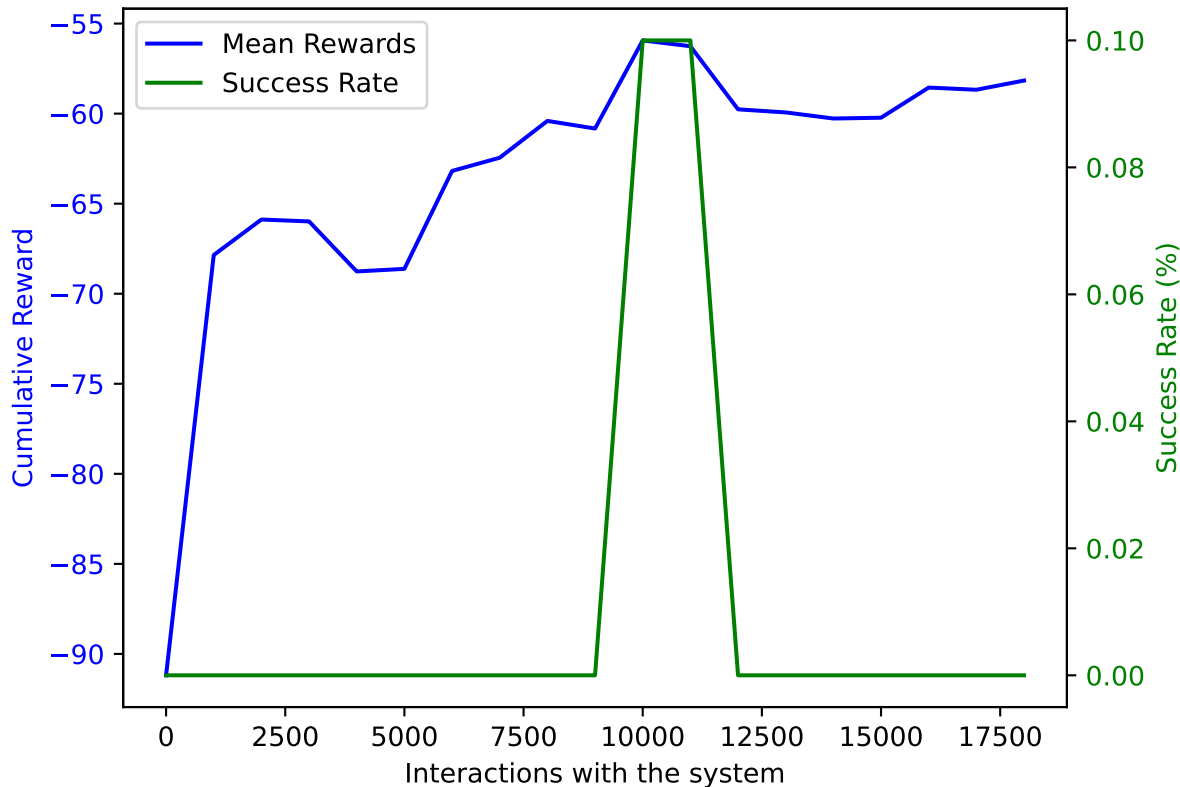
PPO on AWAKE with DoF: 5 and trained on 18000 samples averaged over 10 validation episodes
