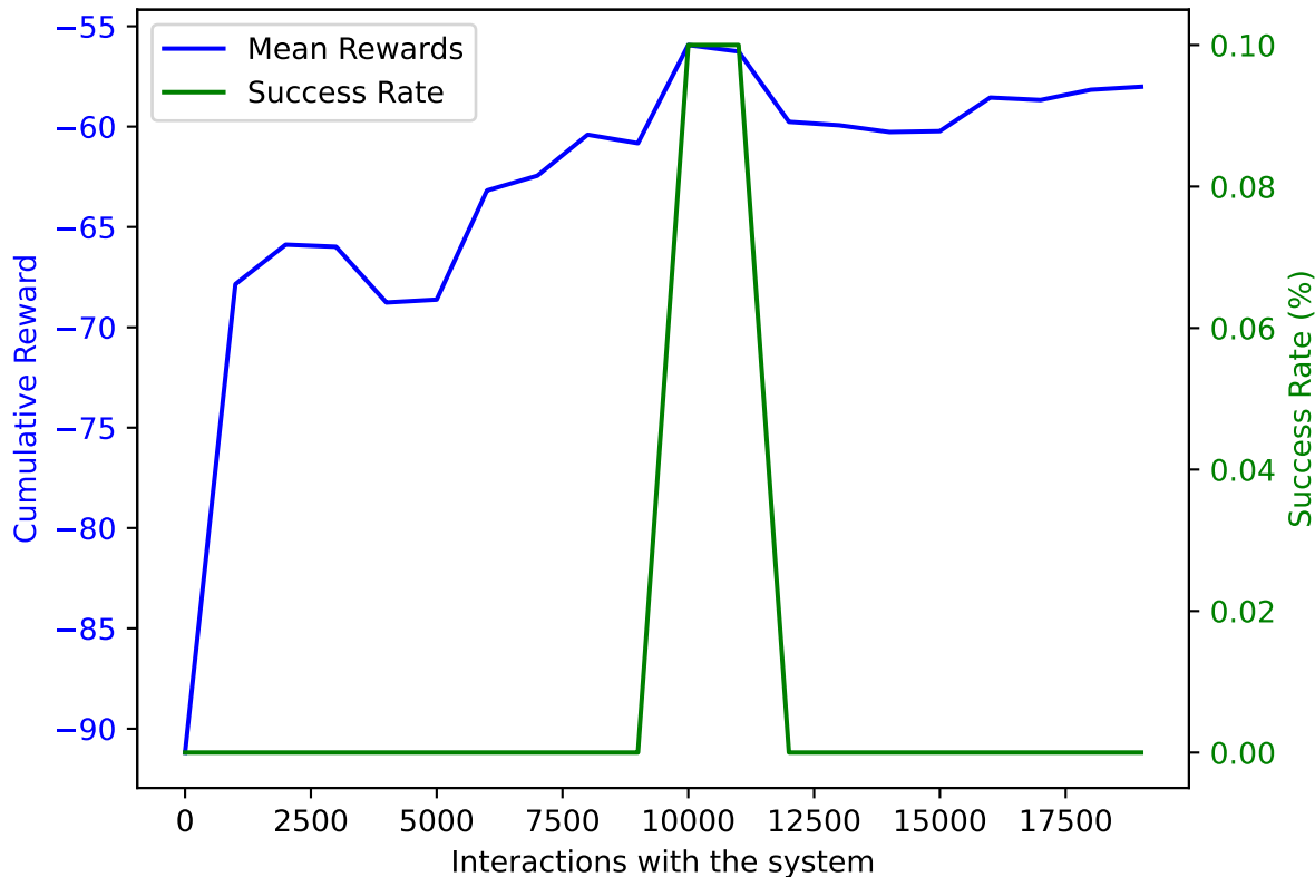
PPO on AWAKE with DoF: 5 and trained on 19000 samples averaged over 10 validation episodes
