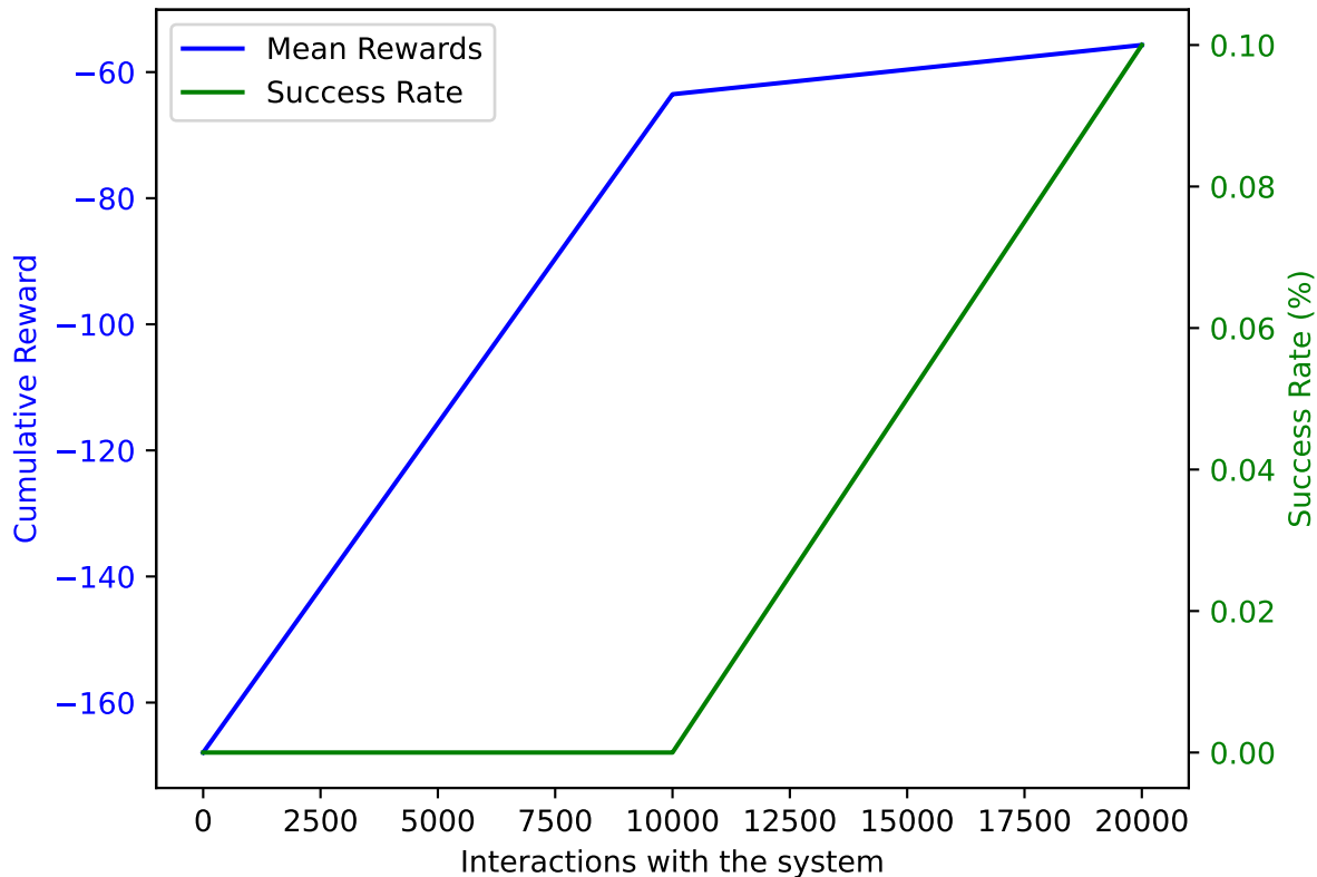
PPO on AWAKE with DoF: 5 and trained on 20000 samples averaged over 10 validation episodes
