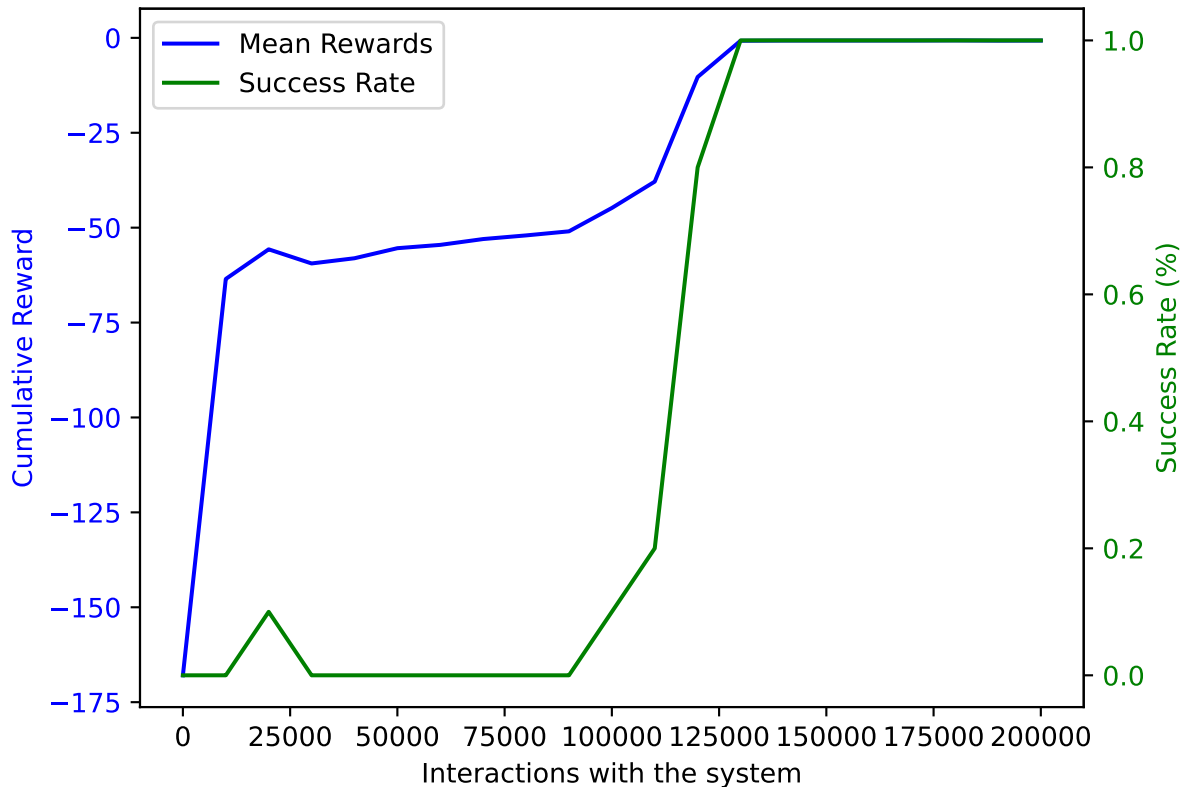
PPO on AWAKE with DoF: 5 and trained on 200000 samples averaged over 10 validation episodes
