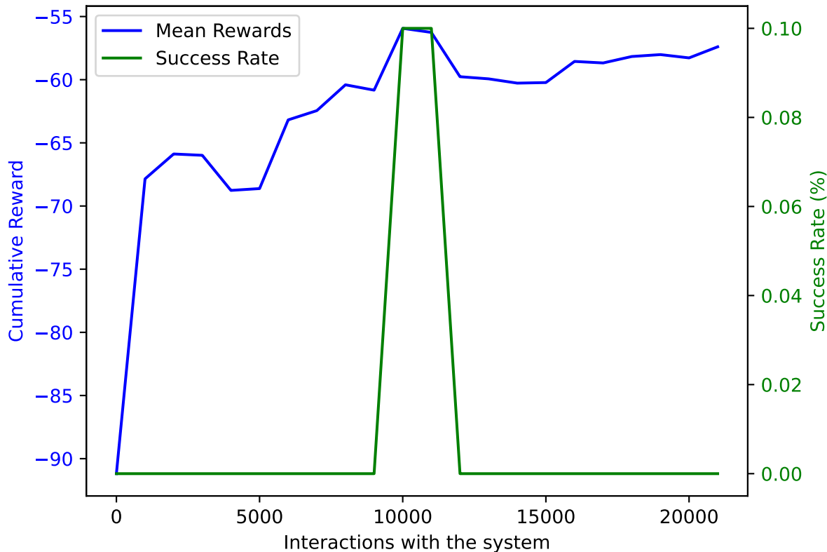
PPO on AWAKE with DoF: 5 and trained on 21000 samples averaged over 10 validation episodes
