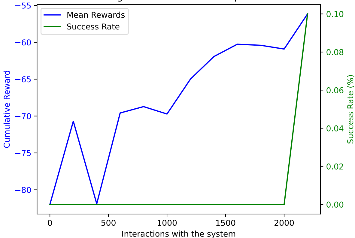
PPO on AWAKE with DoF: 5 and trained on 2200 samples averaged over 10 validation episodes
