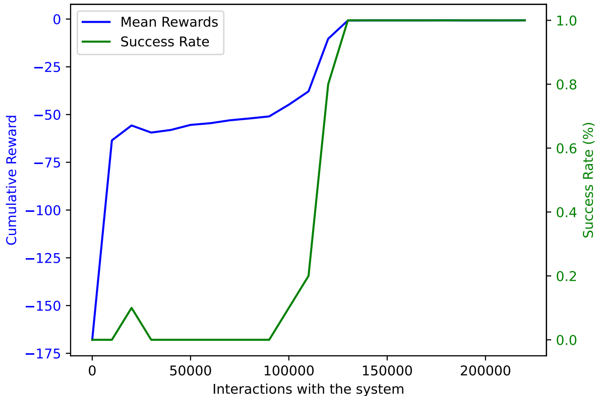
PPO on AWAKE with DoF: 5 and trained on 220000 samples averaged over 10 validation episodes
