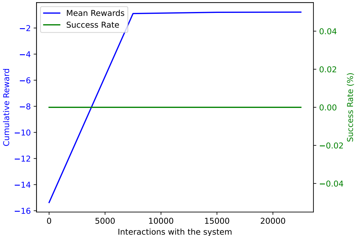
PPO on AWAKE with DoF: 5 and trained on 22500 samples averaged over 10 validation episodes
