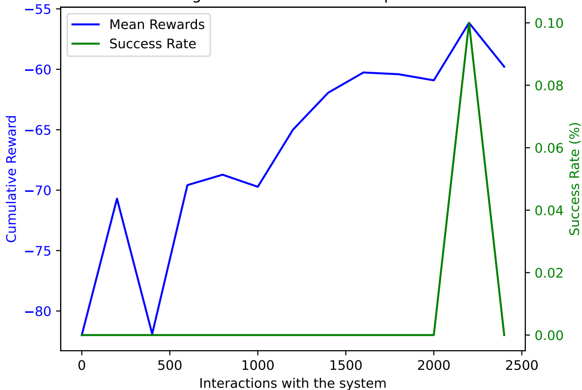
PPO on AWAKE with DoF: 5 and trained on 2400 samples averaged over 10 validation episodes
