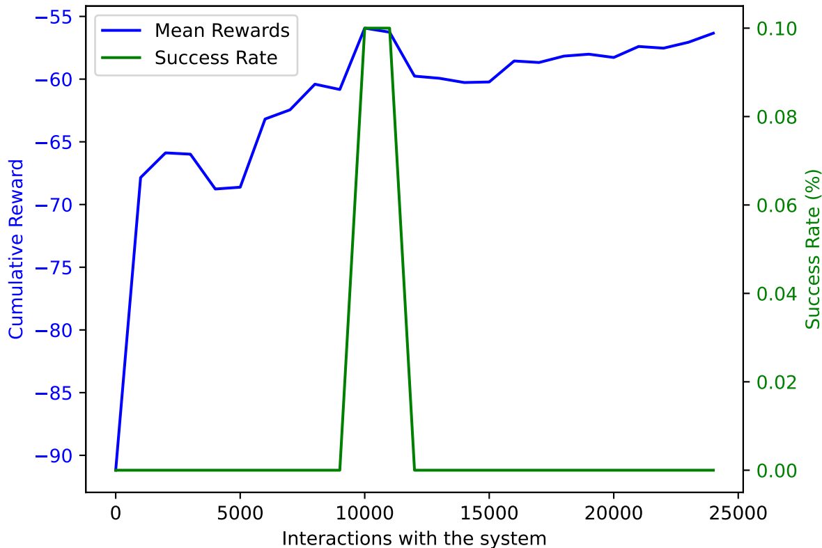
PPO on AWAKE with DoF: 5 and trained on 24000 samples averaged over 10 validation episodes
