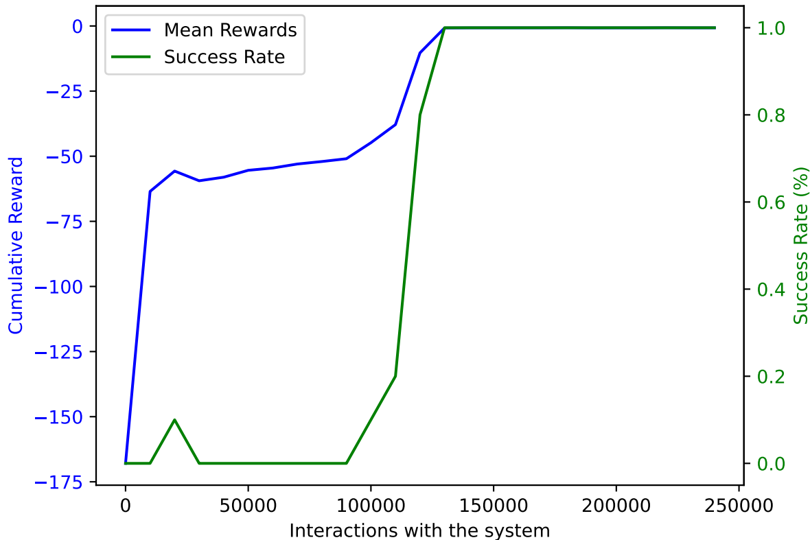
PPO on AWAKE with DoF: 5 and trained on 240000 samples averaged over 10 validation episodes
